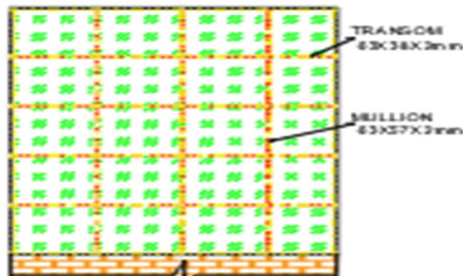
ELEVATION AT B-B
