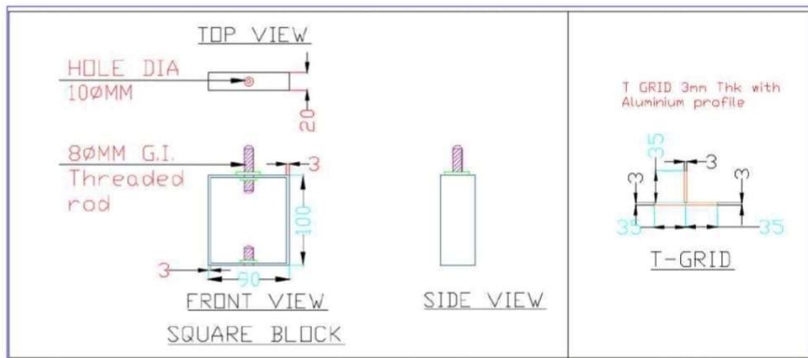
DETAIL - X PLAN & SECTIONAL VIEWS FOR SUPPORTING SYSTEM OF MODULAR FALSE CEILING
