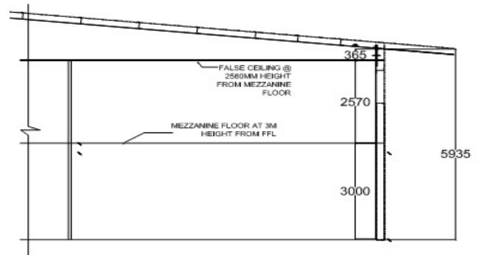
HALF SECTIONAL ELEVATION
