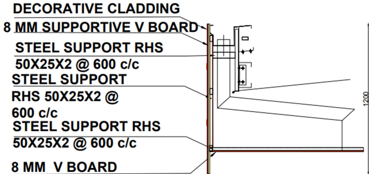
VIEW A
