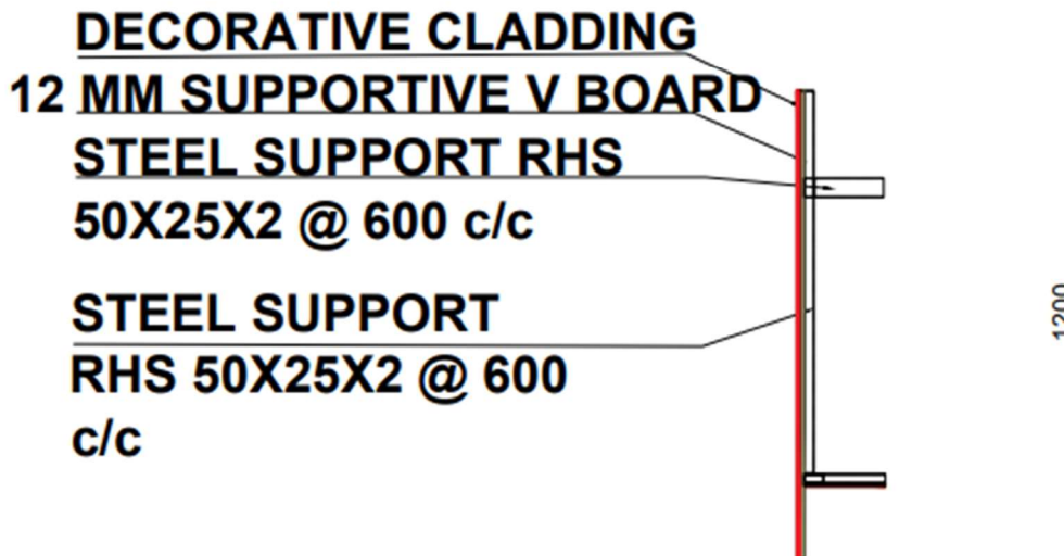
VIEW B
