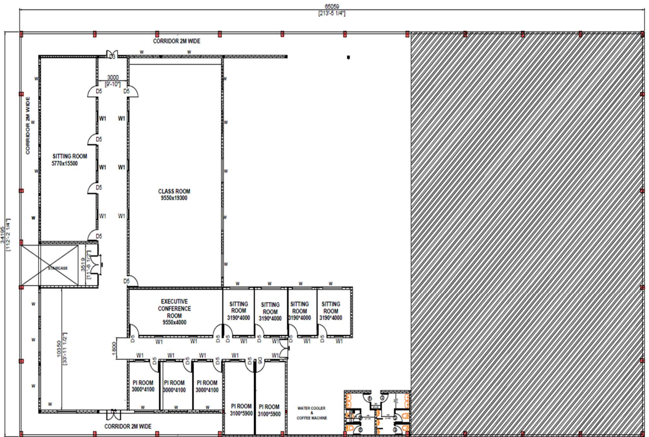
Layout Drawing of First Floor
