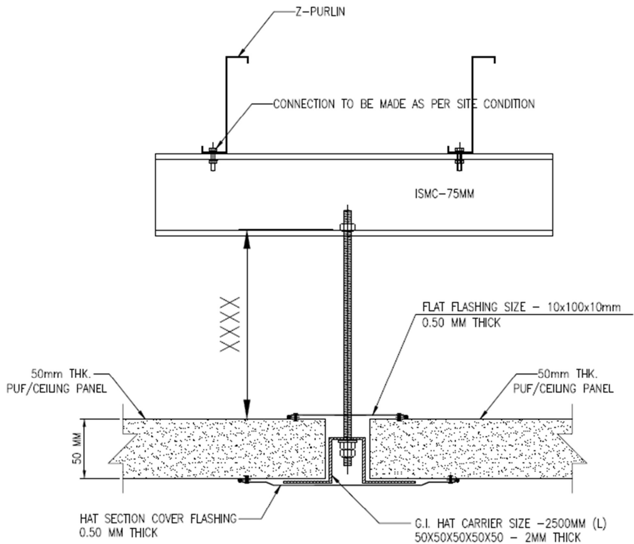
Ceiling Panel to Ceiling Panel Fixing Details With Suspending Arrangement
