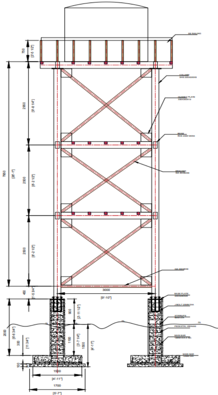
SECTIONAL VIEW A-A
