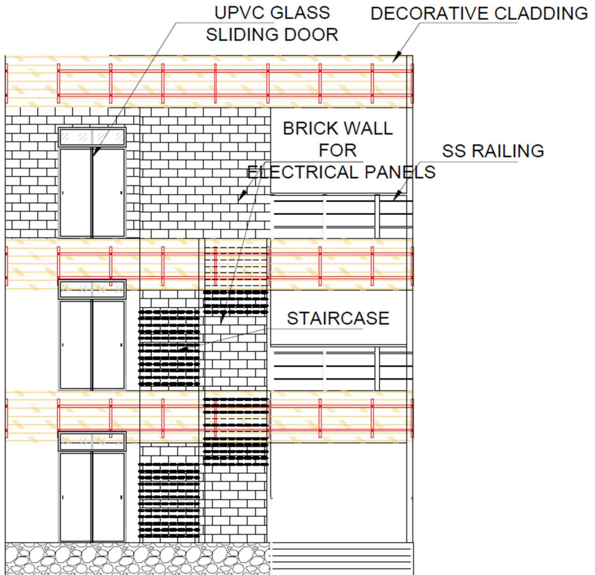
VIEW B-B
