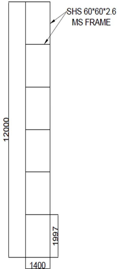
TYPICAL ELEVATION OF JALLI
