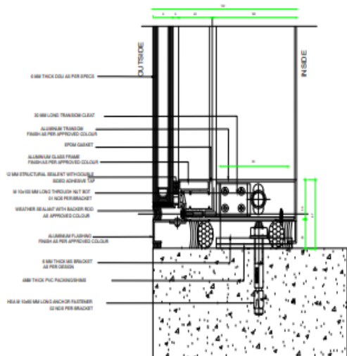
TYPICAL BOTTOM DETAIL
