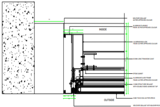
TYPICAL END DETAIL
