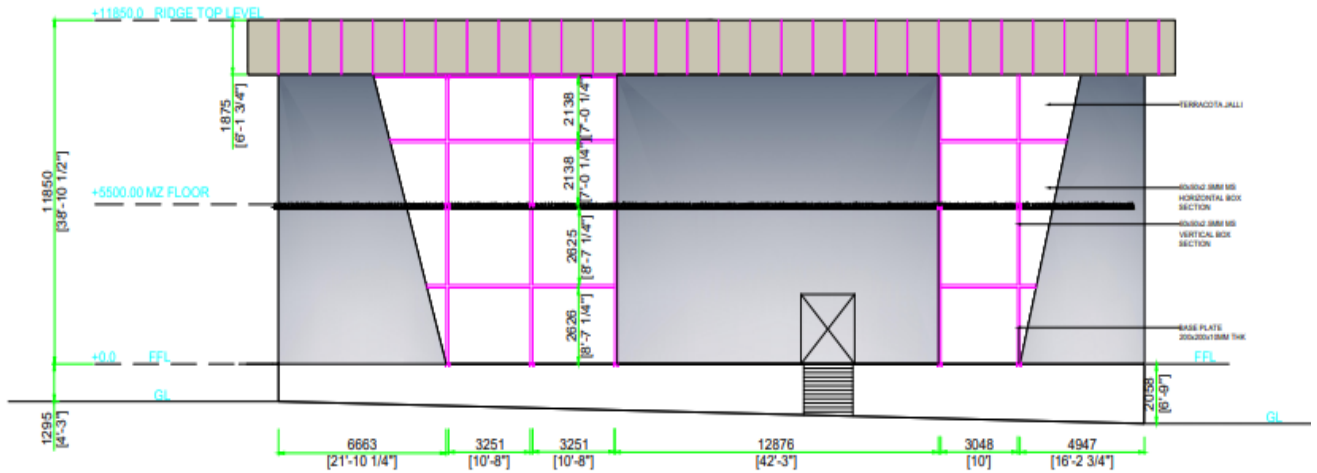
Elevation (Front /West)
