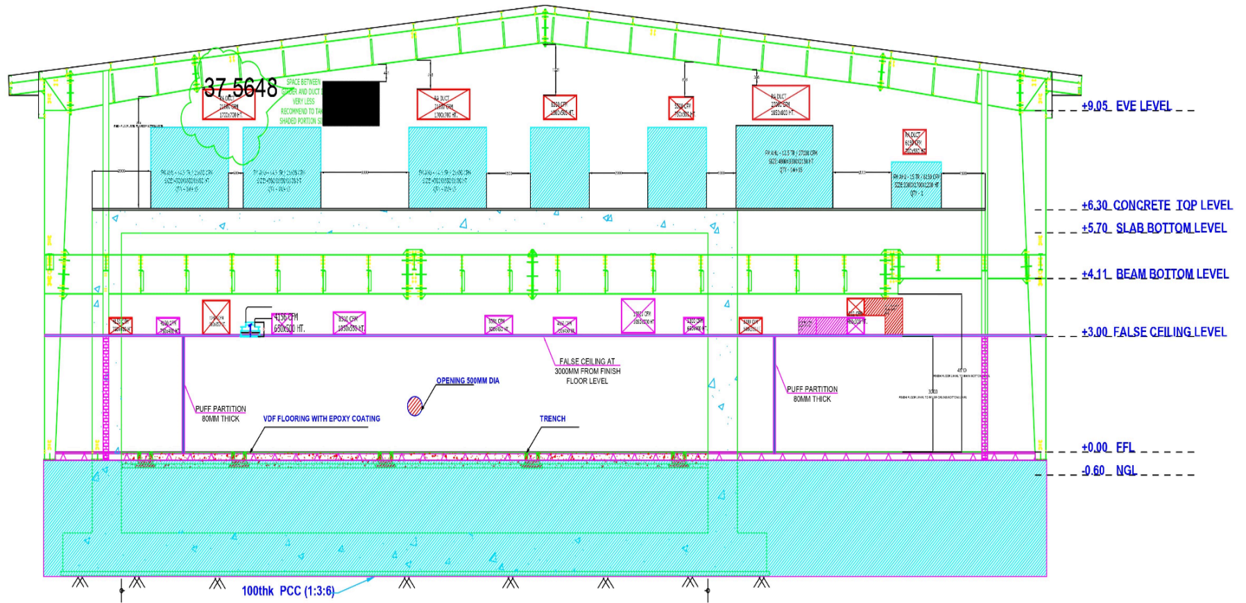
VIEW B-B
