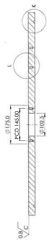
SECTION H-H
