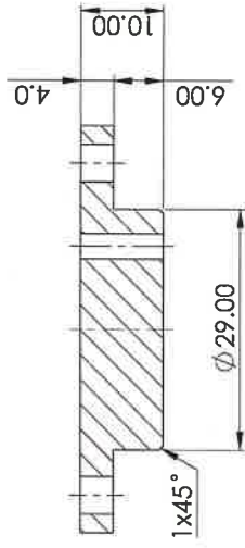
SECTION H-H
