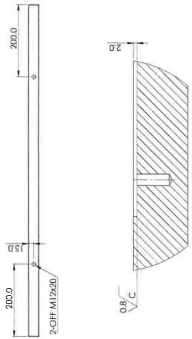
DETAIL L SCALE 1:1
