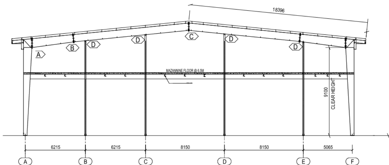
CROSS SECTION ALONG GRID - 12
