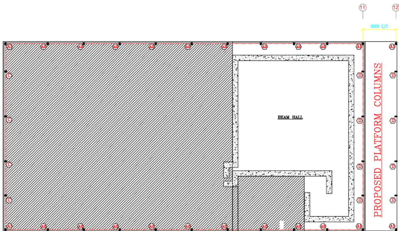
ANCHOR BOLT SETTING PLAN
