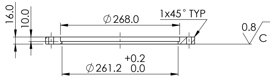
SECTION Q-Q
