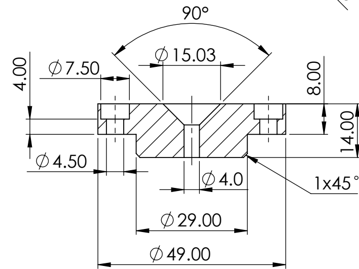
SECTION F-F
